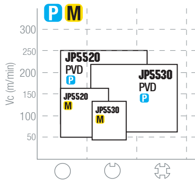
GRADES APPLICATION CHART
