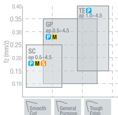
CHIPBREAKERS APPLICATION CHART
