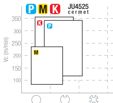
CHIPBREAKERS APPLICATION CHART
